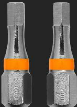
HEX BIT Hex bit insert HEX4 L 25 2pcs in pack 11-01-373
